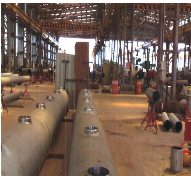
Gas Pipeline for Reliance at Kakinada for KG Basin Cross country Pipeline
